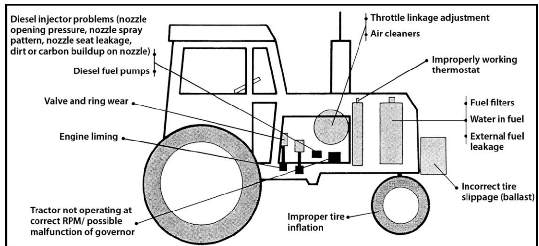
Figure 1. Factors influencing reduced fuel efficiency on a diesel tractor ( http://attra.ncat.org/attra-pub/PDF/consfuelfarm.pdf )
